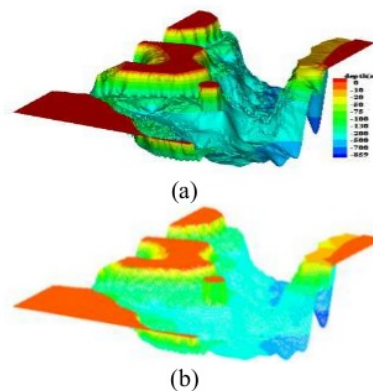
Figure 3. The 3D of the Bunaken strait with water depth: (a) Bathymetry and (b) Meshes.
