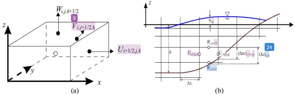
Figure 1. Schematic diagram of computational mesh and notations
