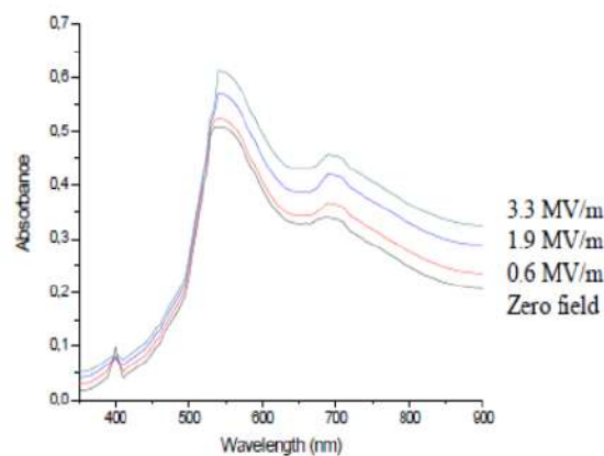
Figure 3. UV-Vis spectra of DR-19 film reflection mode for electric field variations
