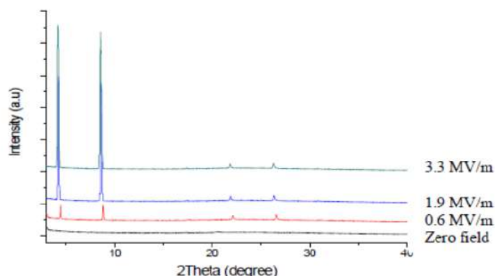
Figure 4. XRD spectra of DR-19 film on silane substrate for electric field variations
