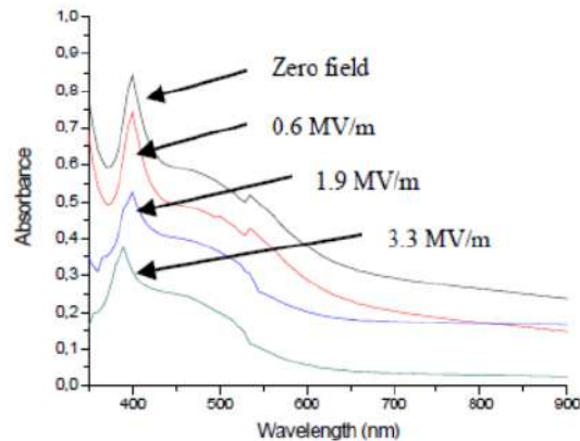
Figure 2. UV-Vis spectra of DR-19 film transmission mode for electric field variations
